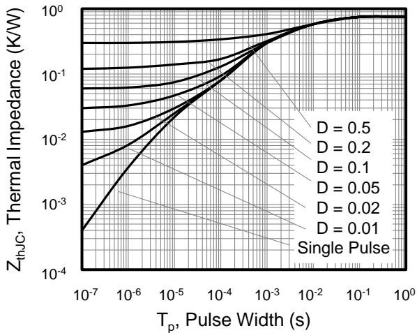
Figure 9. Transient Thermal Impedance TO-220/TO-3P
